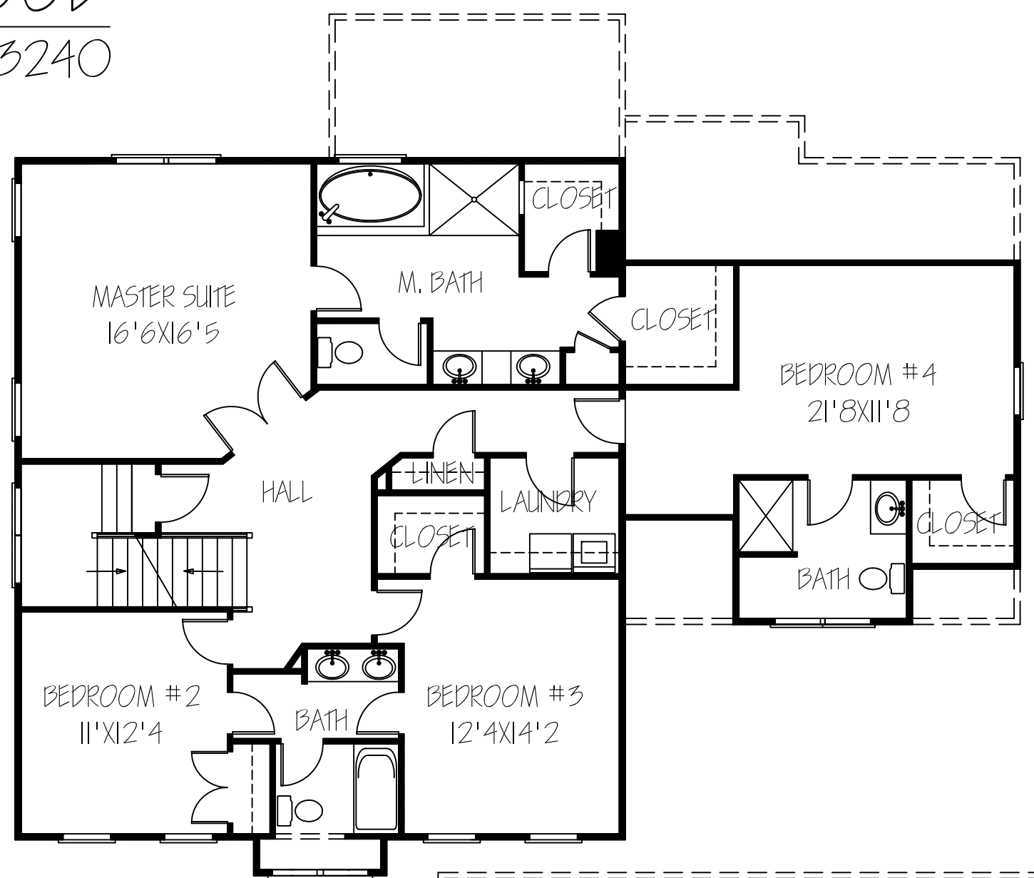
SECOND FLOOR
