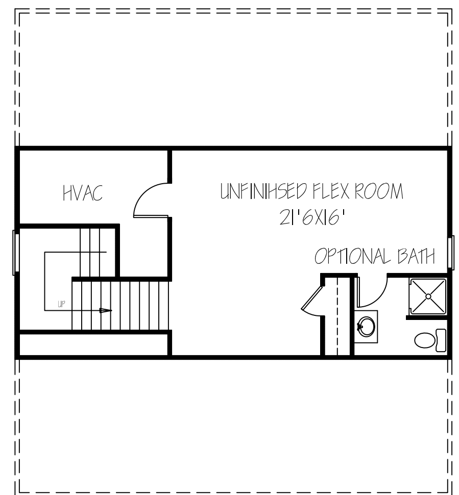
THIRD FLOOR WALK UP ATTIC
